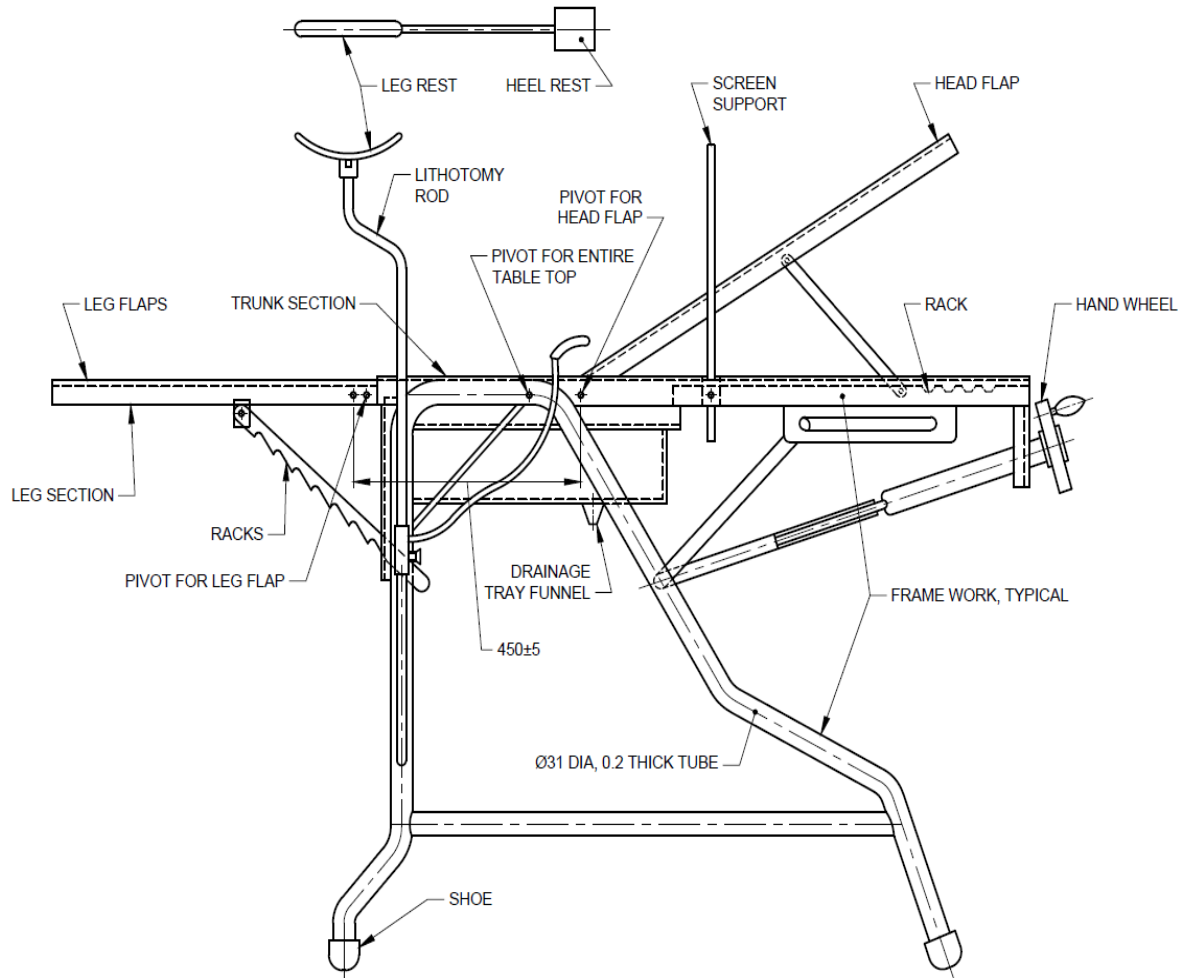
Fig. 1 GENERAL PURPOSE NON-HYDRAULIC OPERATION TABLE
